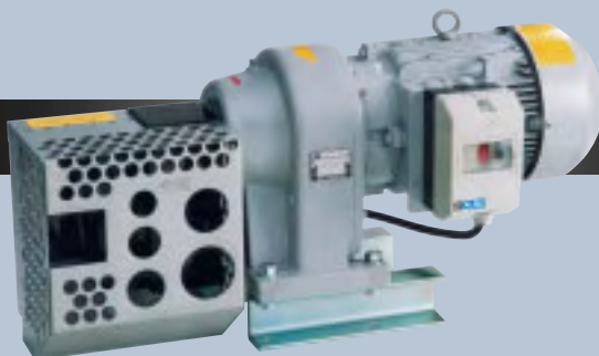
Type AL 1-2U Notching combination with sink outflow. Electric motor (2,2 kW)
